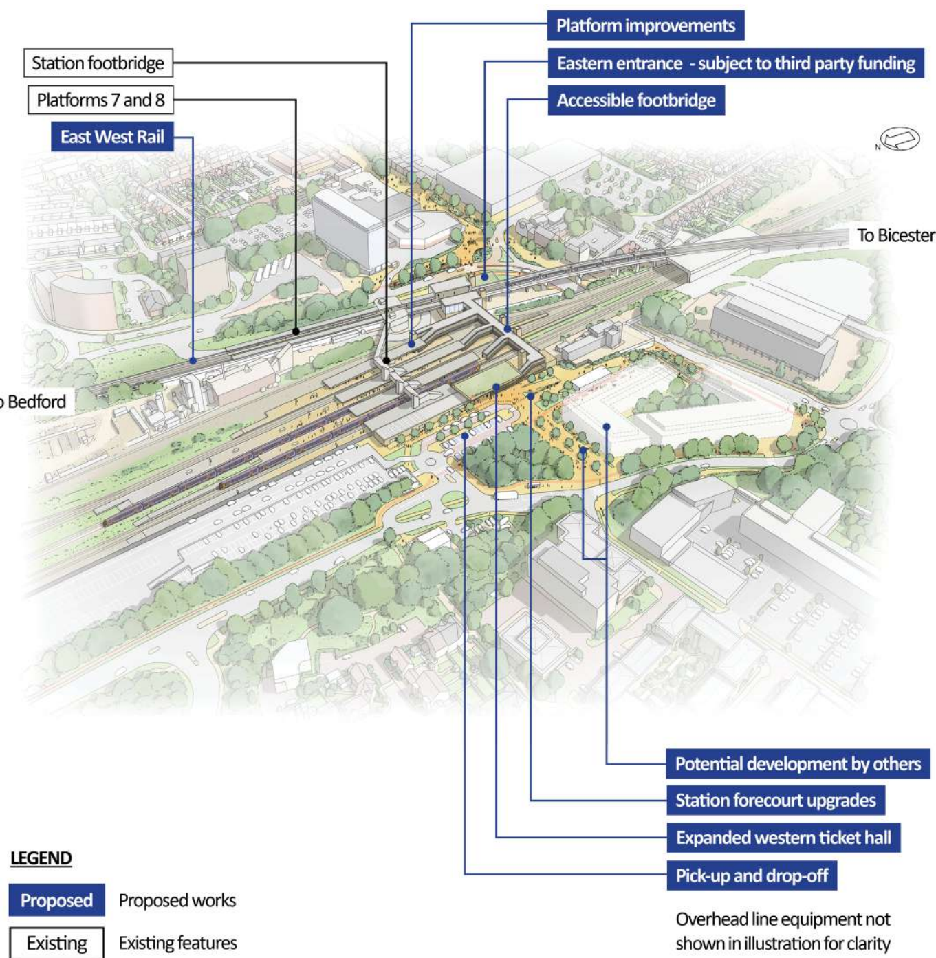
Figure 31: An indicative aerial illustration of Bletchley station
