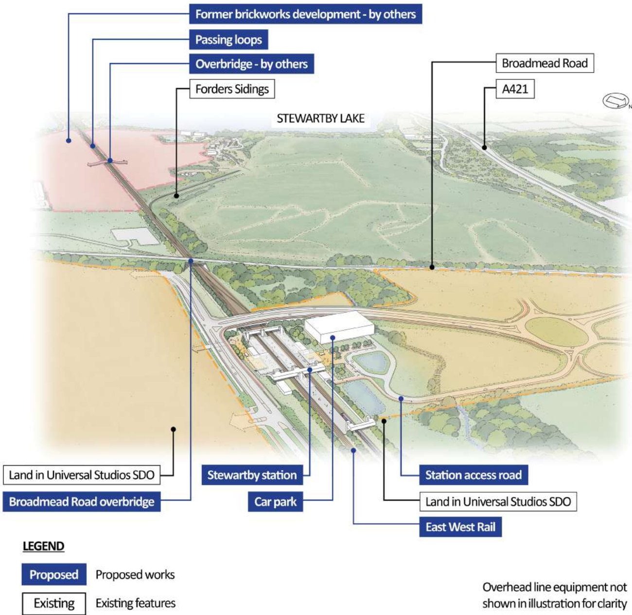
Figure 46: An indicative aerial illustration of the new Stewartby station including loops south of the station
