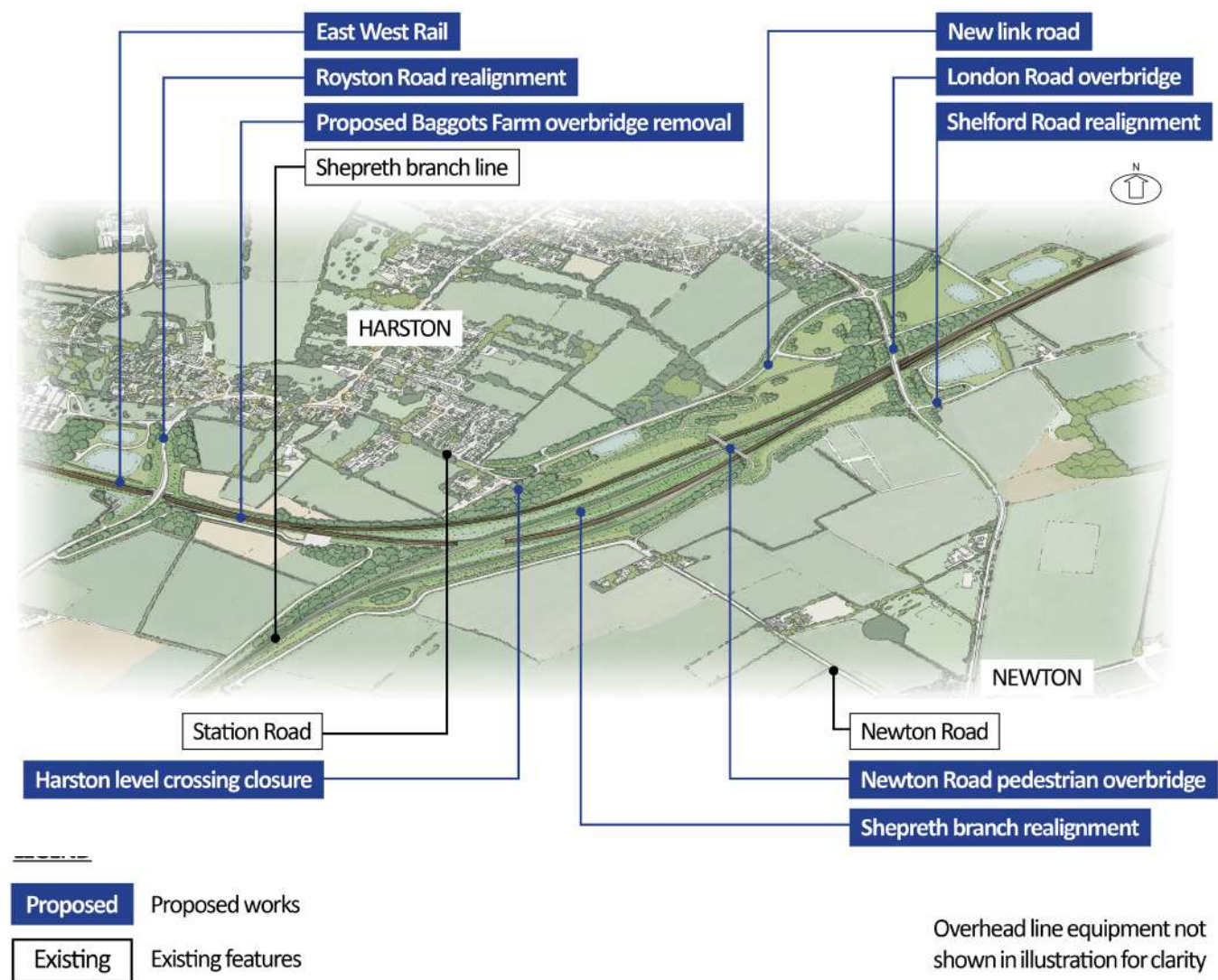
Figure 89: An indicative aerial illustration of the preferred connectivity solution between Newton and Harston
